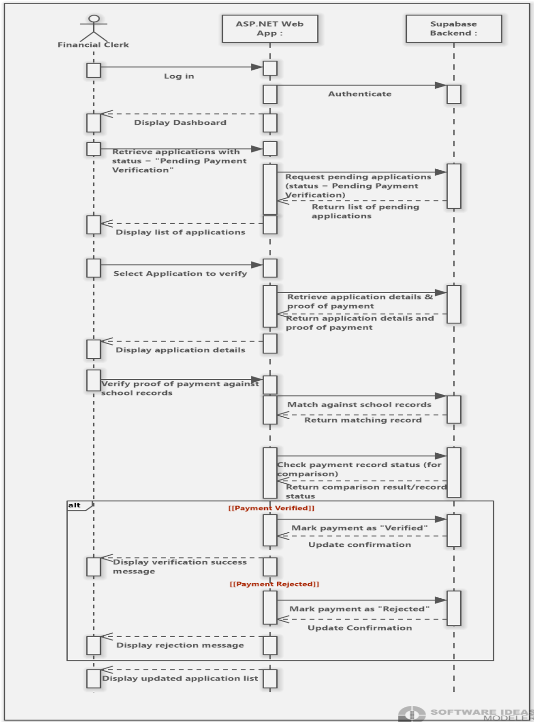
Sequence Diagram 3 – Verify Proof of Payment (ASP.NET)
